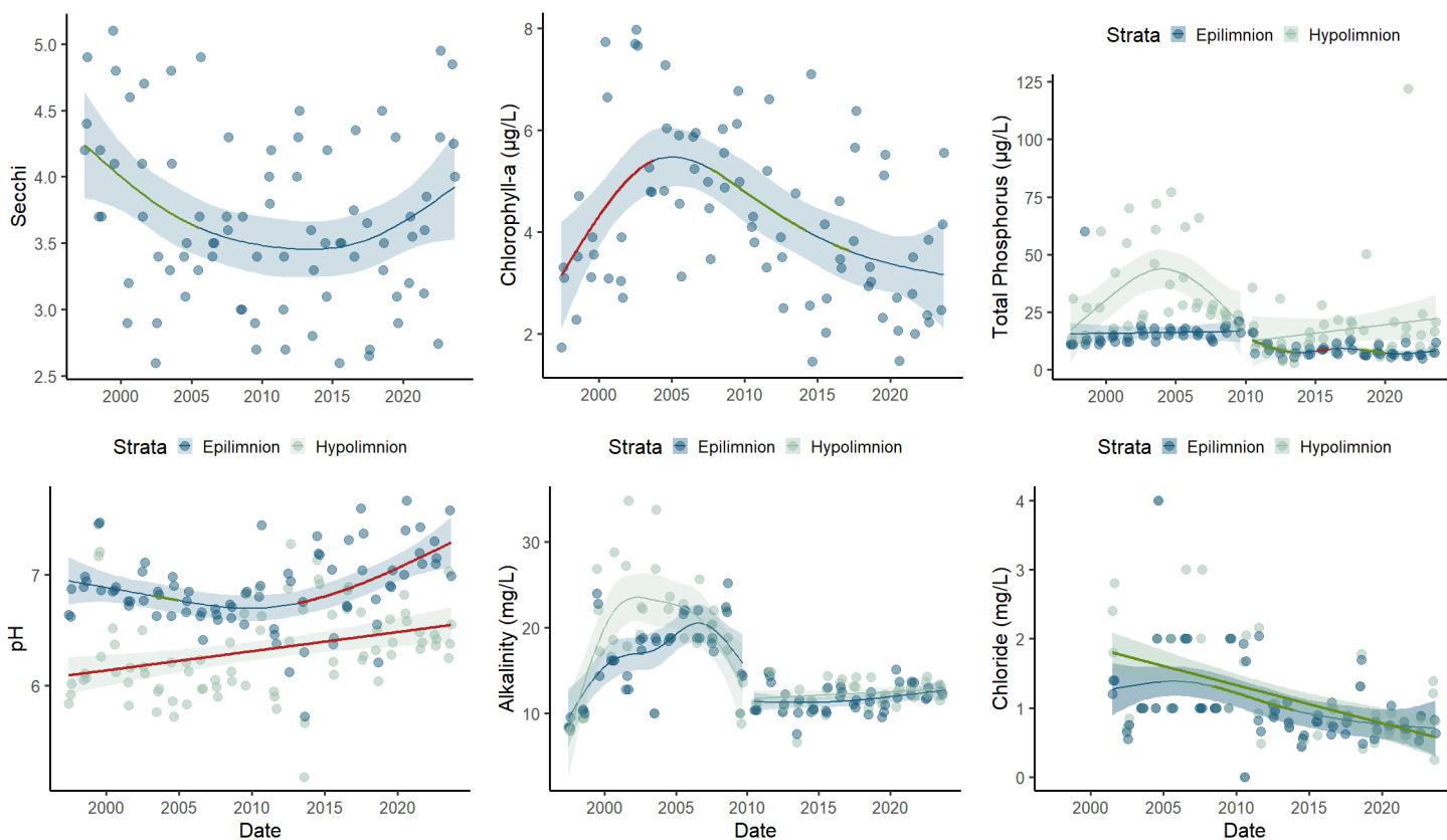
Figure 5. Data for key water quality indicators in Clear Pond, 1997-2023. Fit lines are generalized additive models with shaded areas representing the 95% confidence interval for the model. Overlaid red lines represent periods with a statistically significant increase, overlaid green lines represent periods with a statistically significant decrease. Areas with no red or green overlaid line represent periods with no statistically significant change. Total phosphorus and alkalinity have a break in the fit models to account for an improvement in laboratory methods.
