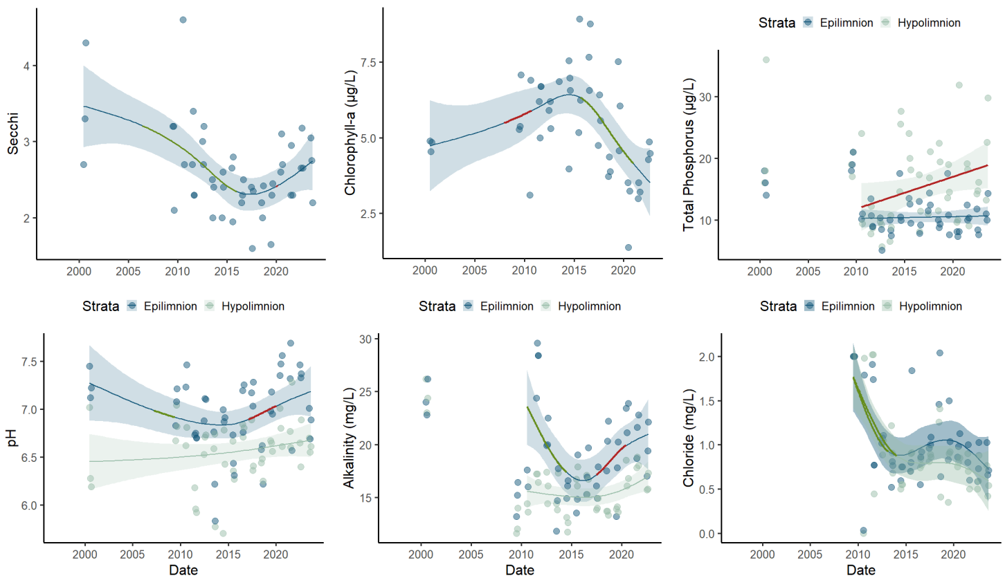
Figure 8. Data for key water quality indicators in Lake Kushaqua, 2001-2023. Regular long-term monitoring began in 2009. Fit lines are generalized additive models with shaded areas representing the 95% confidence interval for the model. Overlaid red lines represent periods with a statistically significant increase, overlaid green lines represent periods with a statistically significant decrease. Areas with no red or green overlaid line represent periods with no statistically significant change. Total phosphorus and alkalinity have a break in the fit models to account for an improvement in laboratory methods.
