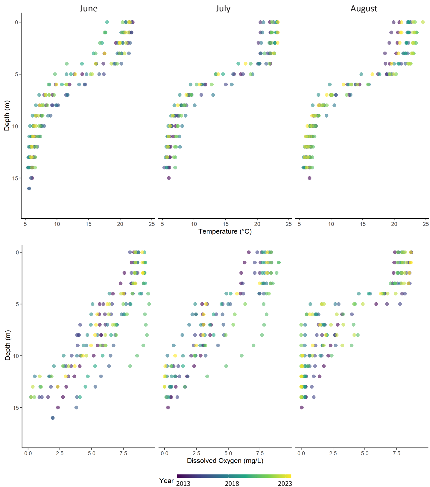
Figure 3. Profiles of temperature and dissolved oxygen in Rainbow Lake from 2013 to 2023. Point color represents the year in which the profile data was collected. Dissolved oxygen concentrations less than 2 mg/L are considered hypoxic and less than 0.5 mg/L are considered anoxic.
