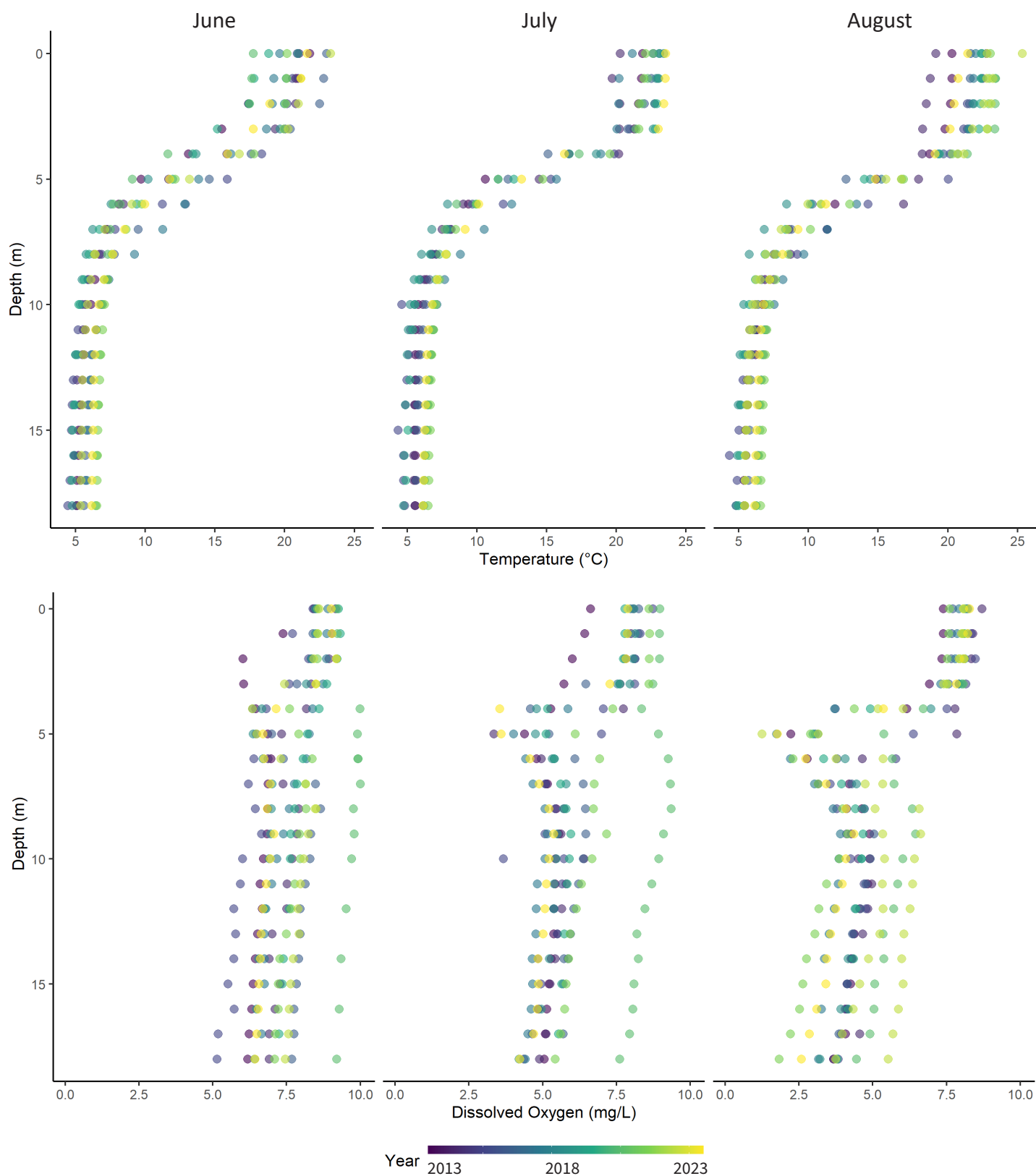
Figure 9. Profiles of temperature and dissolved oxygen in Lake Kushaqua from 2013 to 2023. Point color represents the year in which the profile data was collected. Dissolved oxygen concentrations less than 2 mg/L are considered hypoxic and less than 0.5 mg/L are considered anoxic.
