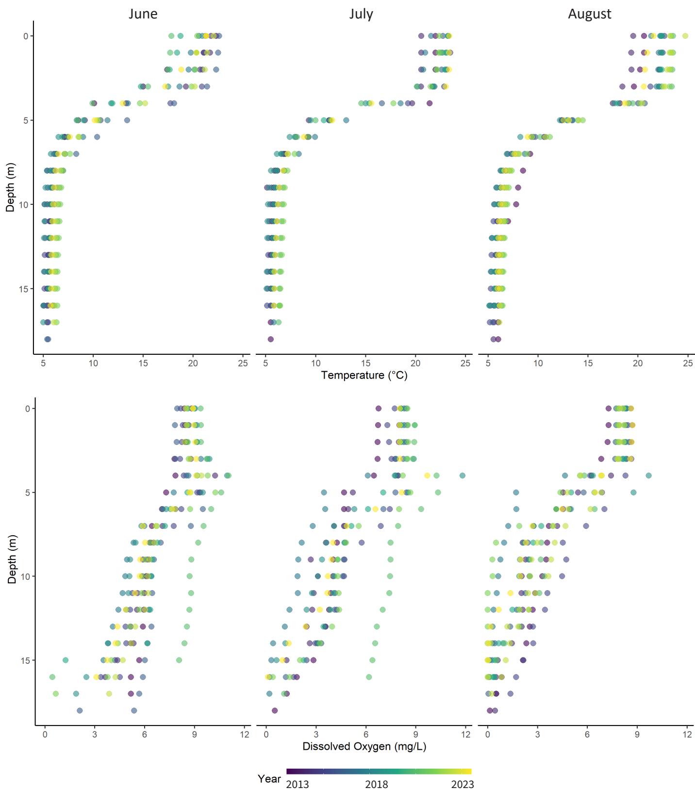
Figure 6. Profiles of temperature and dissolved oxygen in Clear Pond from 2013 to 2023. Point color represents the year in which the profile data was collected. Dissolved oxygen concentrations less than 2 mg/L are considered hypoxic and less than 0.5 mg/L are considered anoxic.
