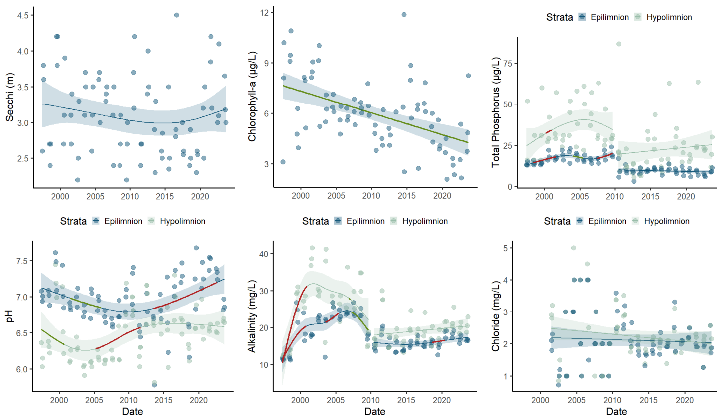
Figure 2. Data for key water quality indicators in Rainbow Lake, 1997-2023. Fit lines are generalized additive models with shaded areas representing the 95% confidence interval for the model. Overlaid red lines represent periods with a statistically significant increase, overlaid green lines represent periods with a statistically significant decrease. Areas with no red or green overlaid line represent periods with no statistically significant change. Total phosphorus and alkalinity have a break in the fit models to account for an improvement in laboratory methods.
